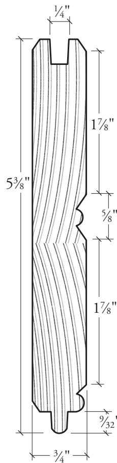
WOTG wide T&G beadboard 16' 30 or TR
