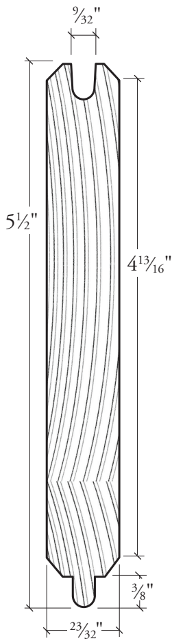
WOTG T&G board 16' 30 or TR
