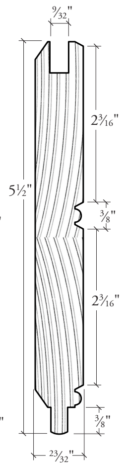
SPBC6 standard T&G beadboard 16' 30 or TR
