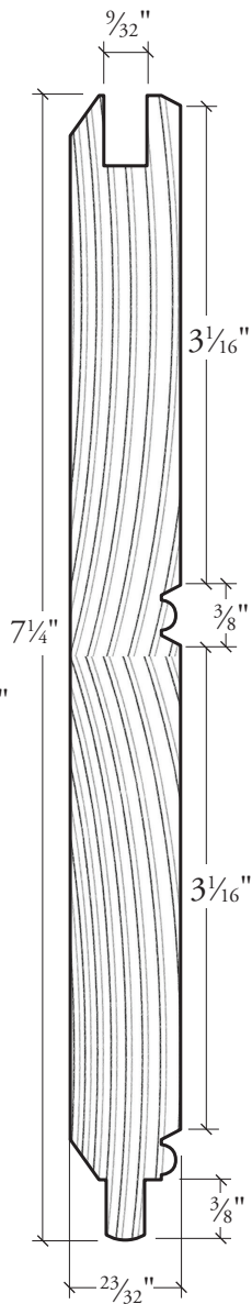
SPBC8 standard T&G beadboard 16' 30
