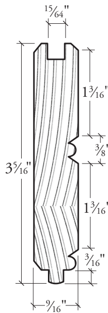
SPBC4 standard T&G beadboard 16' 30 or TR
