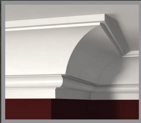
DCR725 1-5/16" x 7-1/4" 18' Lengths Projection: 5-1/4" Height: 5-1/8"
